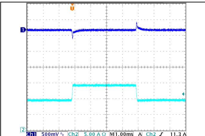
Figure 5: Output voltage response to step-change in load current (50%-75%-50% of I out (max); dI/dt = 0.1 A/μs). Load cap: 1 μF ceramic and 15 μF tantalum capacitors. Ch 1: V out , Ch 2: I out (5 A/div).
