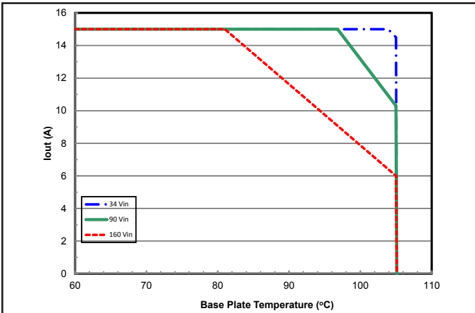
Figure 3: Maximum output current vs. base plate temperature.
