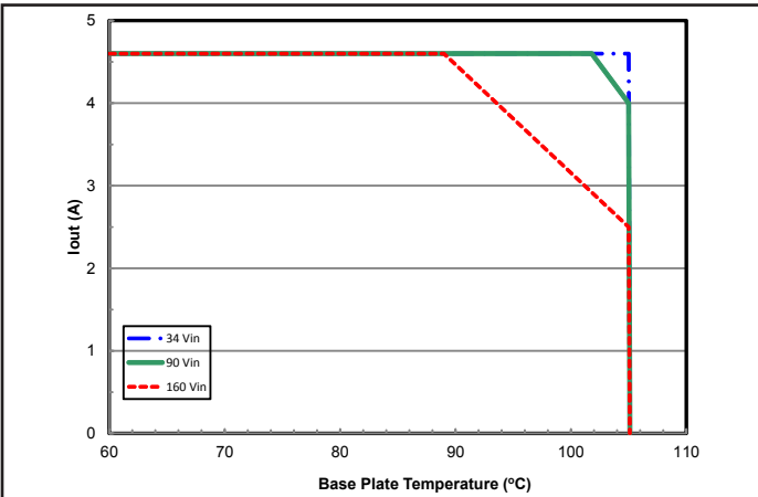
Figure 3: Maximum output current vs. base plate temperature.
