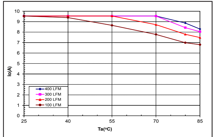
Figure 4: Encased Converter (0.5" heatsink) max. output current derating vs. ambient air temperature for airflow rates of 100 LFM through 400 LFM. Airflows across the converter from input to output (nominal input voltage).
