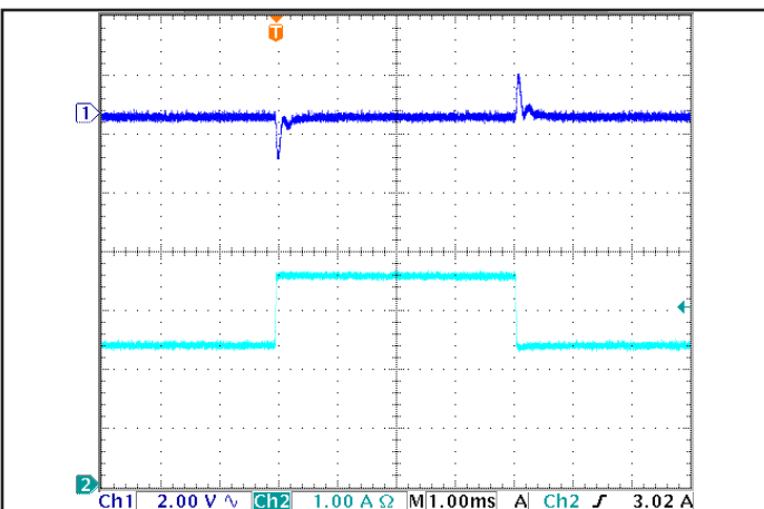
Figure 5: Output voltage response to step-change in load current (50%-75%-50% of I out (max); dI/dt = 0.1 A/μs). Load cap: 1 μF ceramic and 15 μF tantalum capacitors. Ch 1: V out , Ch 2: I out (1 A/div)
