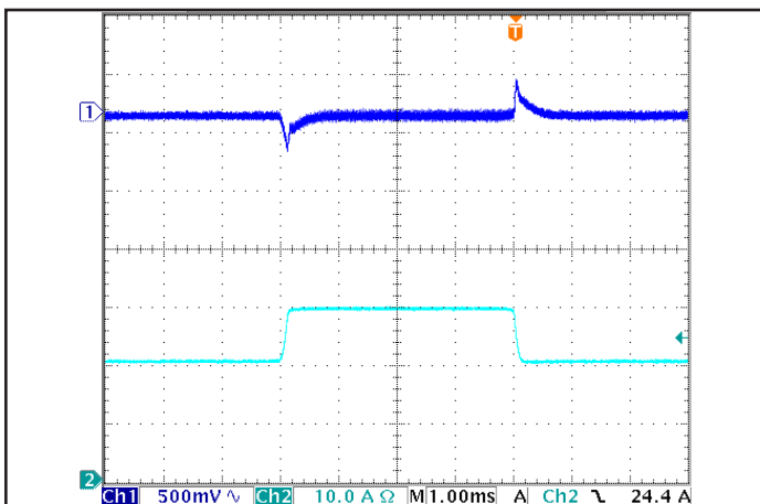
Figure 5: Output voltage response to step-change in load current (50%-75%-50% of I out (max); dI/dt = 0.1 A/μs). Load cap: 1 μF ceramic and 15 μF tantalum capacitors. Ch 1: V out , Ch 2: I out (10 A/div)
